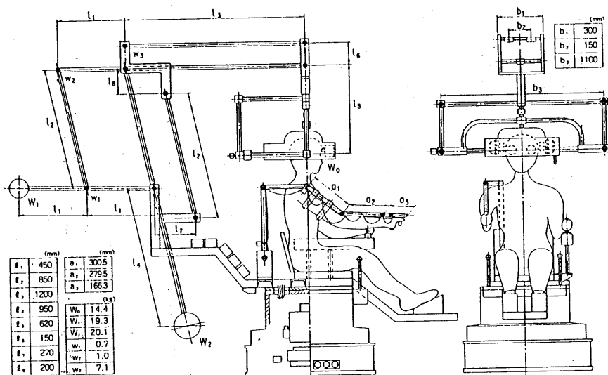
Fig. 4 Schematic diagram of the tele-existence master system.
