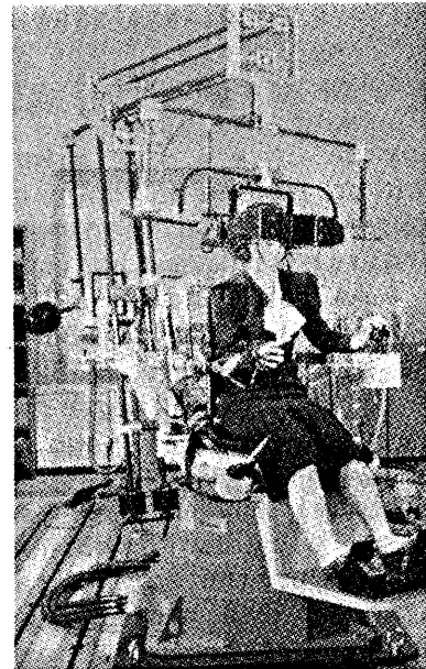
Fig. 3 General view of the tele-existence master system.
