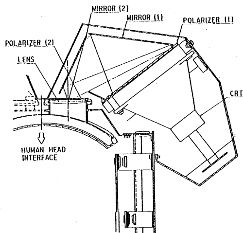
Fig. 6 Visual display design (right eye side).
