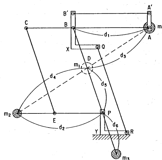
Fig. 5 Parallel link mechanism.
