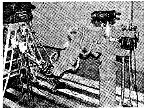
Fig. 1 General view of the anthropomorphic slave robot.
