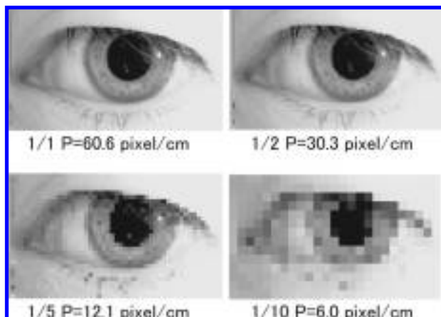
Figure 9. Down-sampled images.
