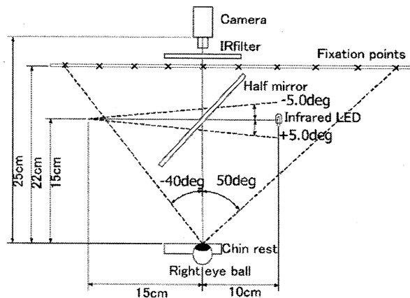
Fig. 4 Experimental arrangement
