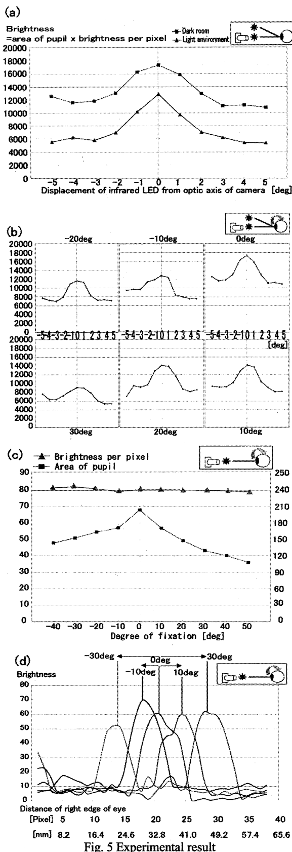
Fig. 5 Experimental result
